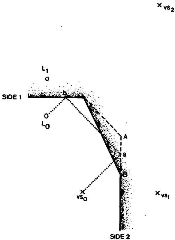
FIG. 6. Although vs_2 is visible in side 1 from the listener position, vs_2 still will not be visible if side 2 extends only to point B. Validating segment a-b of the sound path requires that virtual listener L_1 look for vs_1 in side 2. L_1 will not see vs_1 if side 2 ends at B.
