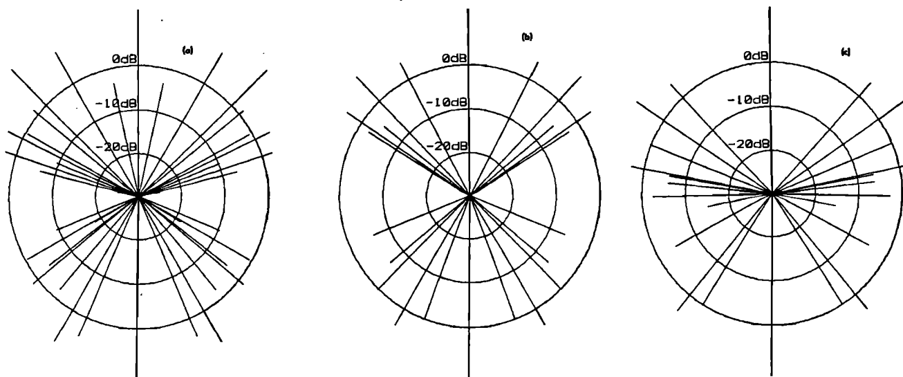
FIG. 11. The polar plots for the same sequence of halls from (a) rectangular to (b) fan to (c) reverse fan emphasize that the lateral sound is more centralized in the fan hall and less in the reverse fan than the rectangular hall.
